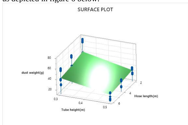
Figure 6. Surface Plot
