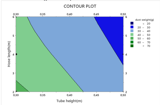
Figure 5. Contour Plot of the Effect between Hose Length and Tube Height to Weight
