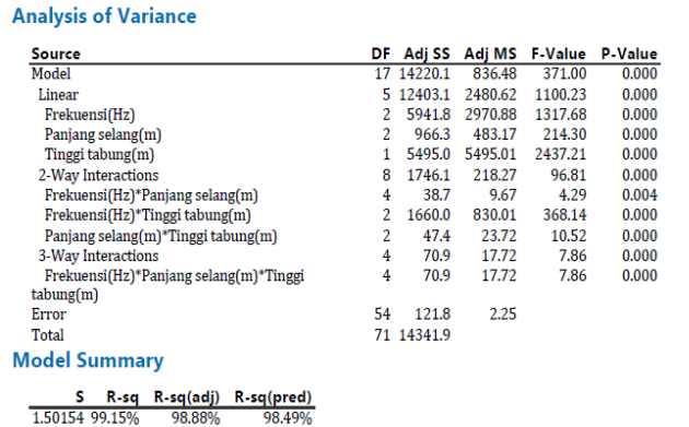
Figure 3. ANOVA results
