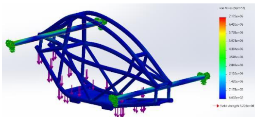
Fig. 6. Stress Value at 1100 N Load
