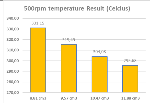
Fig. 7 the Combustion Chamber Temperature Data Testing at 500 RPM
