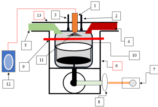
Fig. 1. Installation scheme
