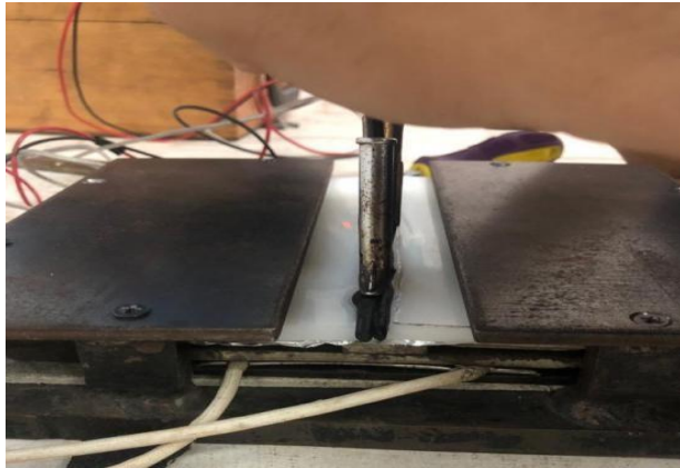
Figure 4. The Hot-Gas Welding Process
