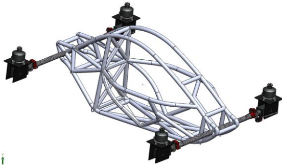
Figure 1 Drone design
