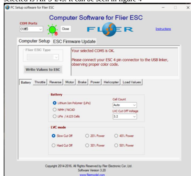
Figure 4 Flier Program
