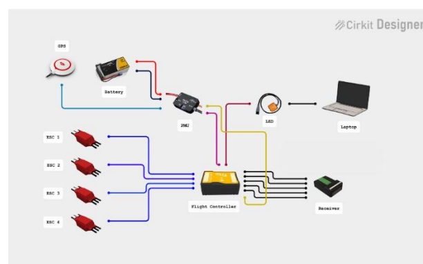
Figure 2 Wiring Flight Controller on ESC
