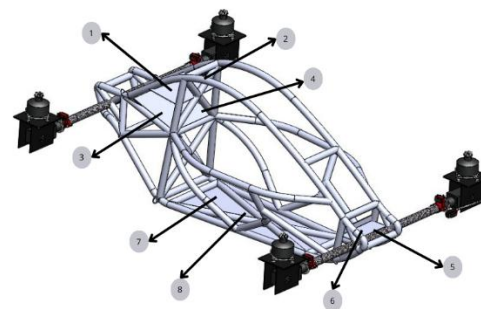
Figure 1 Desain Quadcopter
