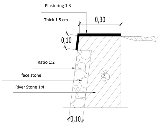
Fig. 3 Cross Section and Stucco Details
