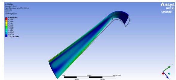
Figure 10. Von Mises Stress on wind speed 7 m/s and elbow width 130 mm
