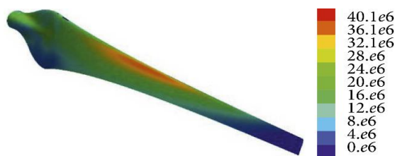
Figure 5: Von Mises Stress evaluation for E-glass-epoxy and basalt-epoxy at 40 m/s using CFD simulation [20]
