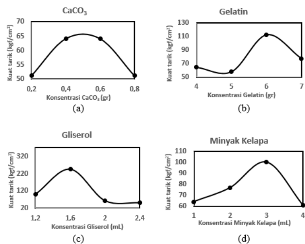
Figure 1 (a) CaCO 3 Single-direction test graph, (b) Gelatin Single-direction test graph, (c) Glycerol Single-direction test graph, (d) Coconut oil Single-direction test graph.
