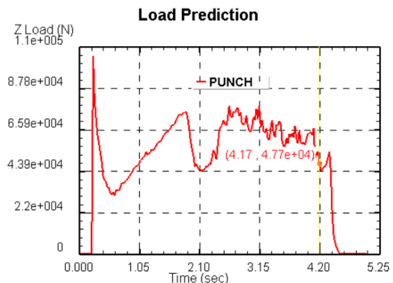
Fig 10. Load prediction for punch of 10 of the 45 degrees angle 5 blank of deep drawing process of aluminium 7075
