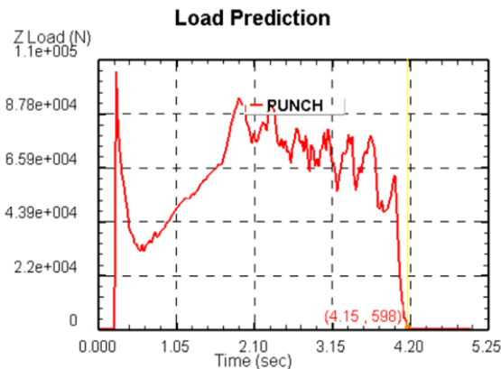
Fig 8. Load prediction for punch of C10 with the 30-degree angle tool blank of deep drawing process of aluminium 7075
