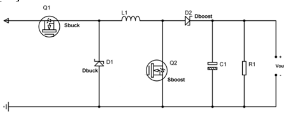
Fig 2. Buck-boost Converter with 2 Switches
