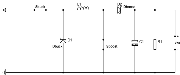
Fig 3. Switch Close
