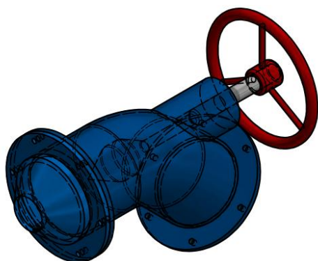
Figure 6. Pelton turbine nozzle.
