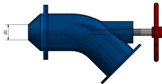
Figure 10. Jet nozzle diameter dimensions.
