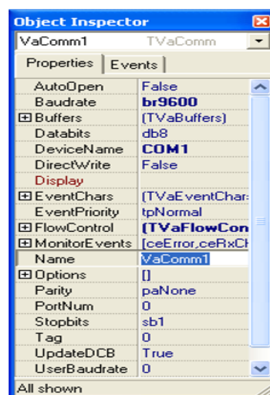
Figure 9 Property Setting Serial Vacomm Delphi.
