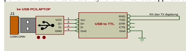
Figure 6 Testing Diagram of USB To TTL Converter
