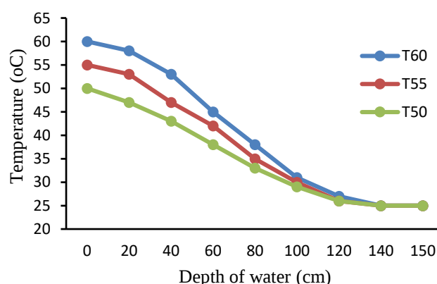
Figure 6 Water temperature in the pool
