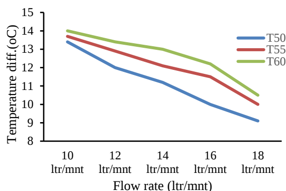
Figure 7 The effect of water discharge on the temperature difference.
