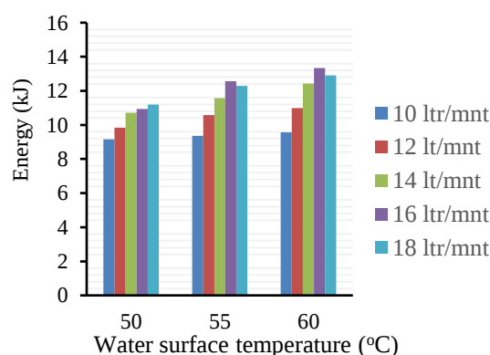
Figure 10. The effect of surface water temperature on the energy released
